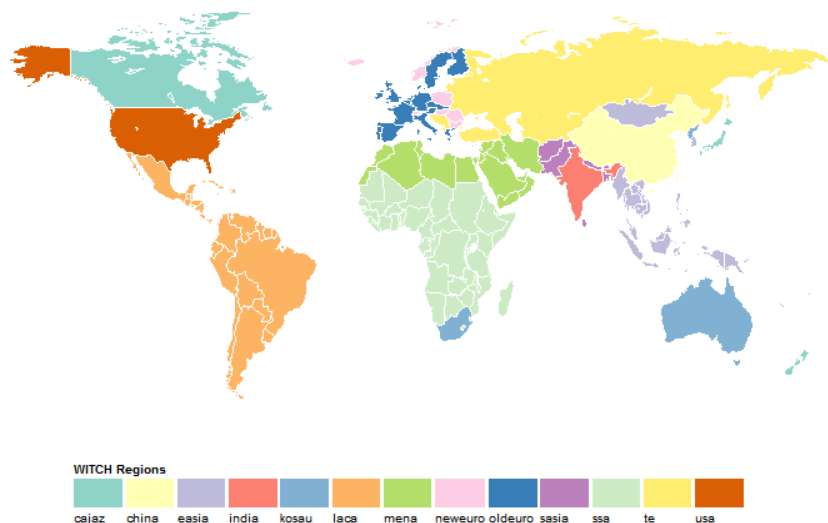
Figure 2.1: WITCH original regions
