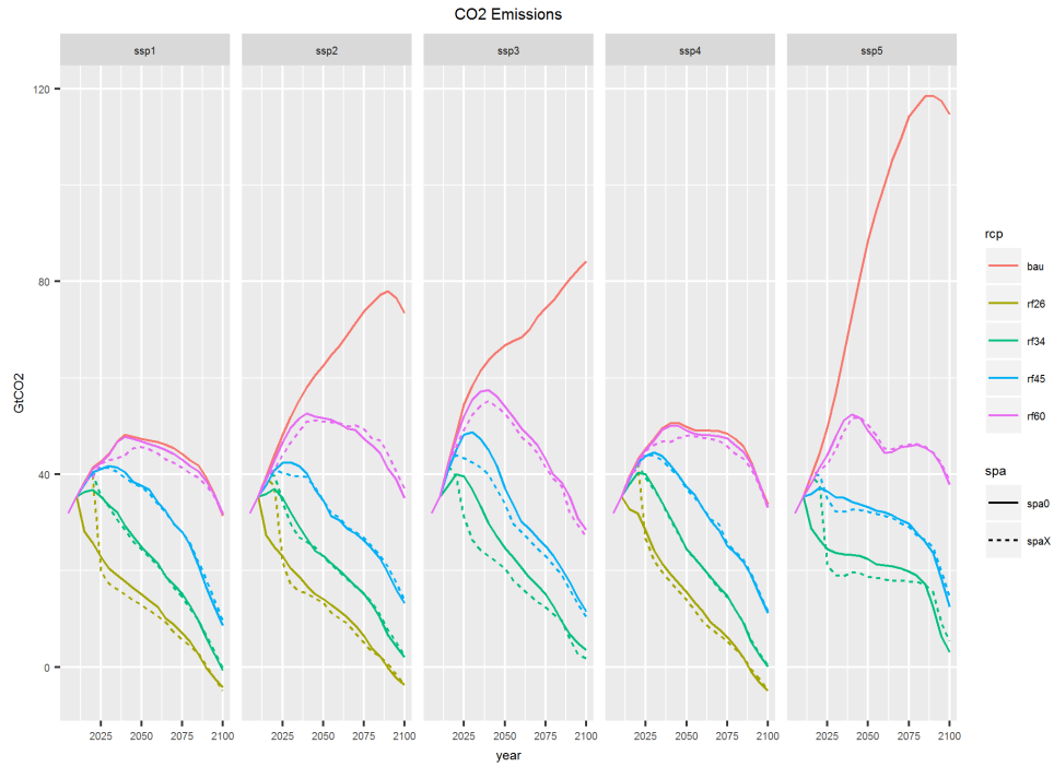
Figure 10.6: CO2 Emissions
