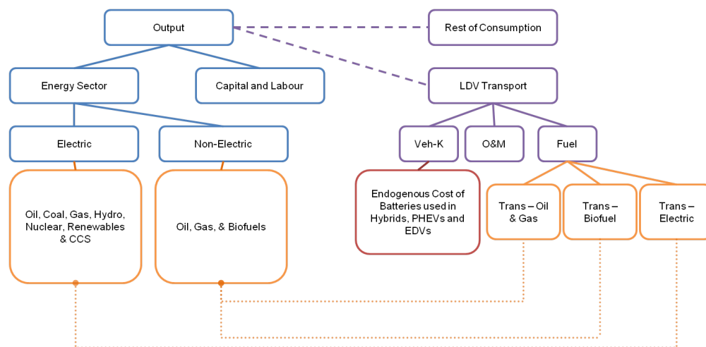
Figure 4.2: Transport Sector Structure
