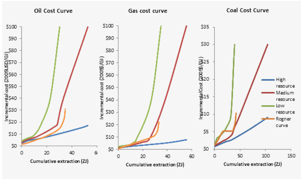
Figure 5.1: ROSE supply curves
