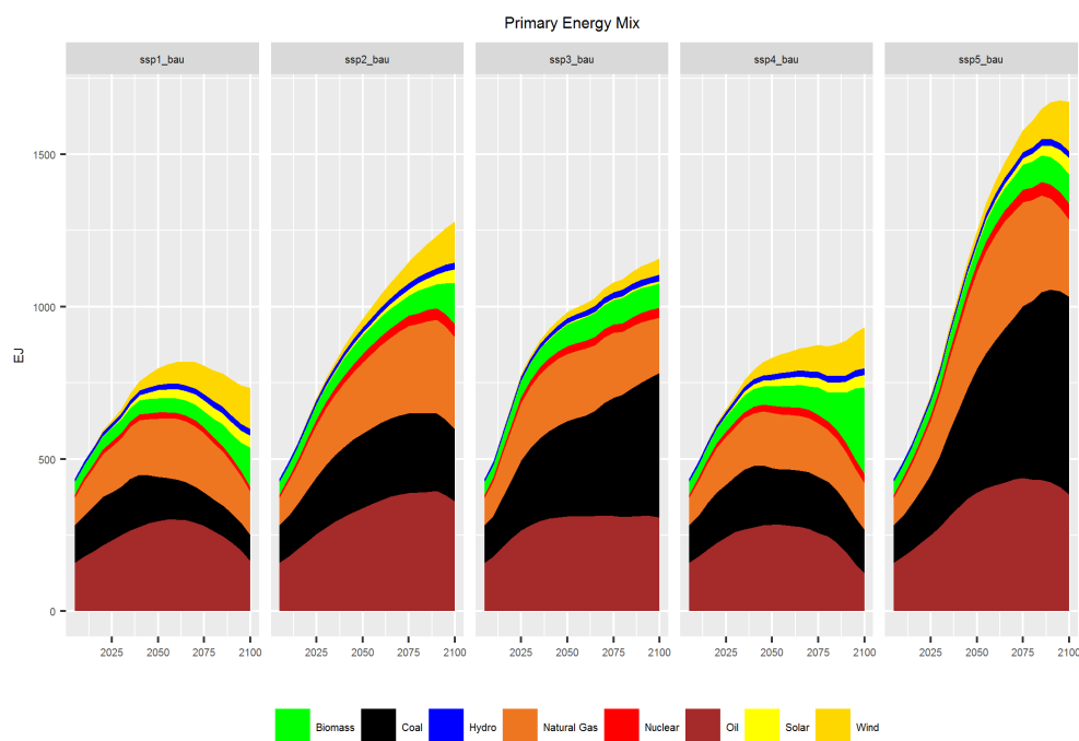
Figure 10.5: Primary Energy Supply
