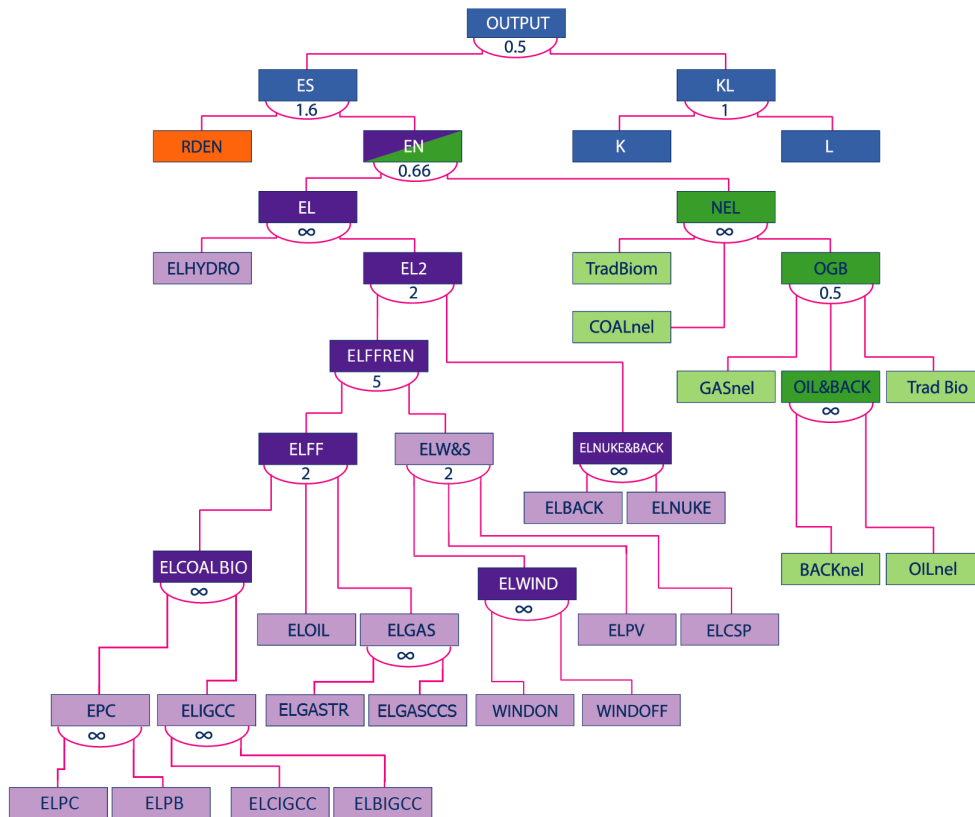
Figure 4.1: CES Production Function of WITCH
