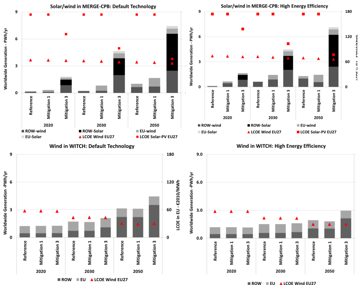
Figure 7. Worldwide generation (PWh/yr) and levelized costs (LCOE, 2010euro/MWh) in Europe for wind and solar-PV power. Results from the MERGE-CPB (upper panel) and WITCH (lower panel) models for the default (left panel) and high energy efficiency (right panel) cases.
