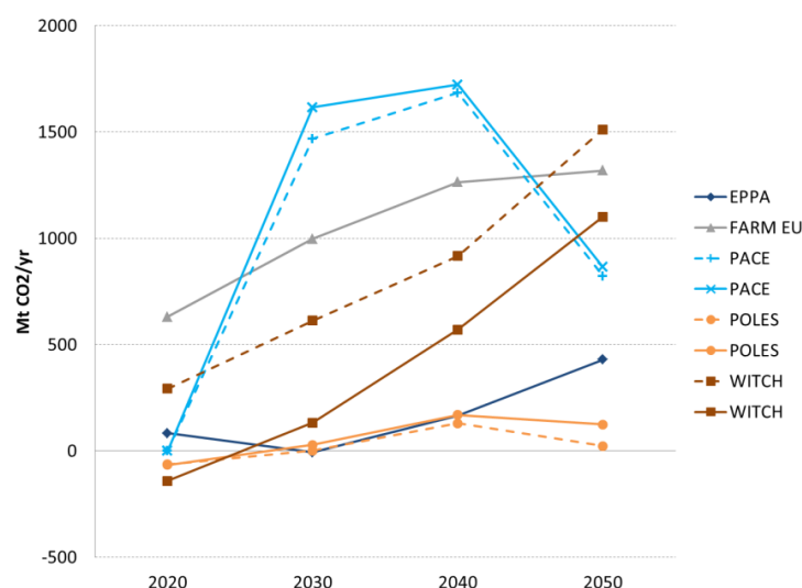
Figure 10. Emission permits purchased by the EU on the international market computed as difference in CO 2 industrial emissions between Mitigation 3 (80%GLOB) and Mitigation 2 (80%FRAG), under default (solid lines) and high energy efficiency technology case (dashed lines).
