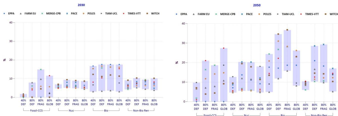
Figure 6. Percentage share of various low carbon energy on total primary energy in 2030 and 2050 for the following models, EPPA, FARM-EU, MERGE-CPB, PACE, POLES, TIAM-UCL, TIMES-VTT, WITCH. TIAM-UCL is not included in the scenarios Mitigation 1 (80%DEF) and Mitigation 2 (80%FRAG).
