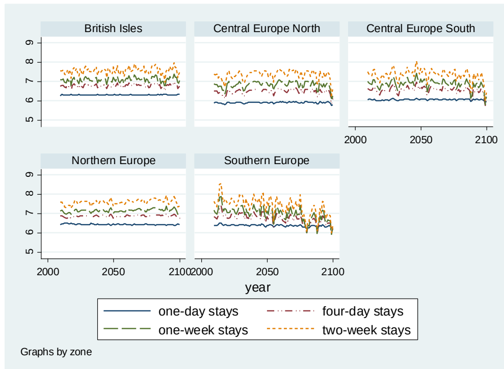
Figure 3: Evolution of the predicted hedonic price index during the spring months: 2010-2099 (average by country and months)
