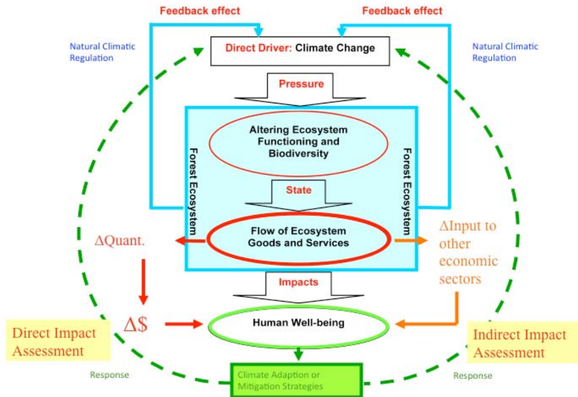
Figure 1. A Conceptual model for the climate change, forest biodiversity and human well-being interactions
