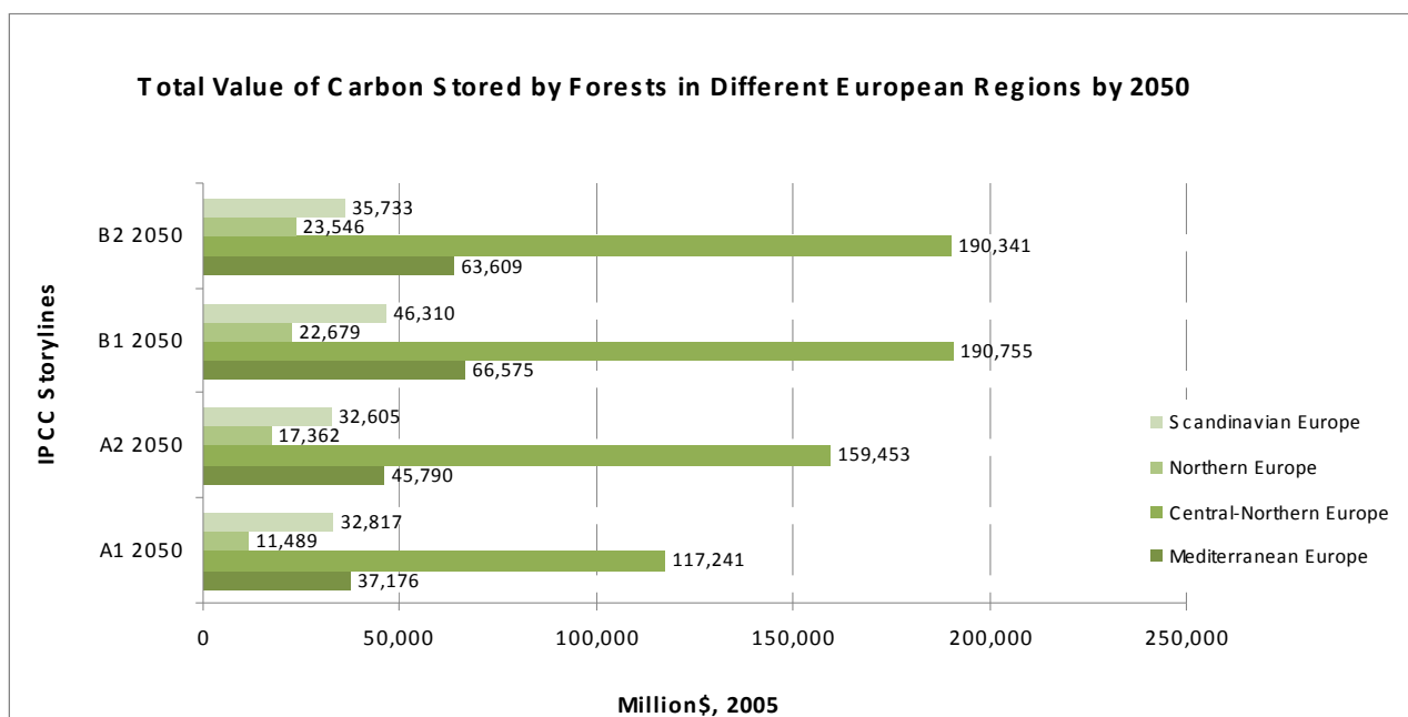
Figure 3 Forest carbon sequestration values
