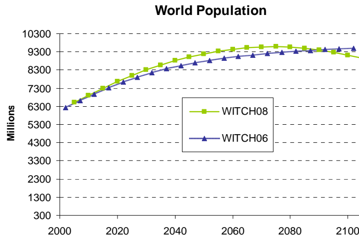
Figure 2: Population dynamics
