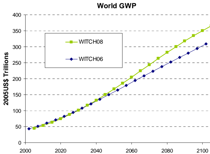
Figure 3: GWP trajectories
