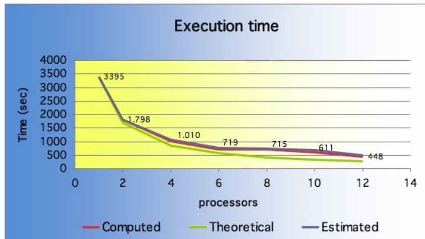
Figure 6: Execution time
