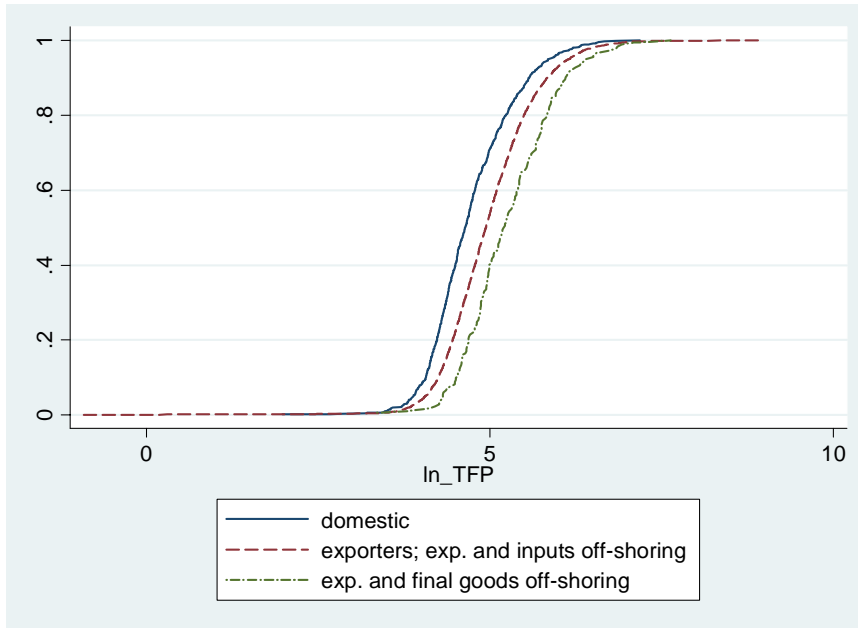
Figure 3: Plot of the cumulative distribution function of TFP: purely domestic, exporters, horizontal off-shorers (Levinsohn-Petrin method; classification based on Question D3.2.1)
