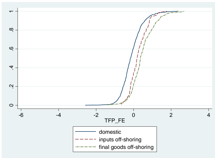
Figure 4: Plot of the cumulative distribution function of TFP: purely domestic, inputs off-shoring, final goods off-shoring (fixed effects method; classification based on Question D3.2.1)
