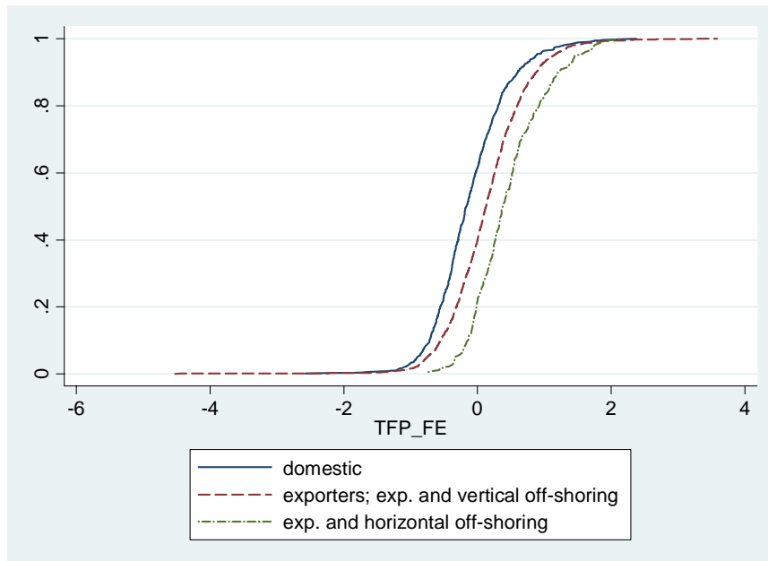
Figure 1: Plot of the cumulative distribution function of TFP: purely domestic, exporters, horizontal off-shorers (fixed effects method; BR classification)
