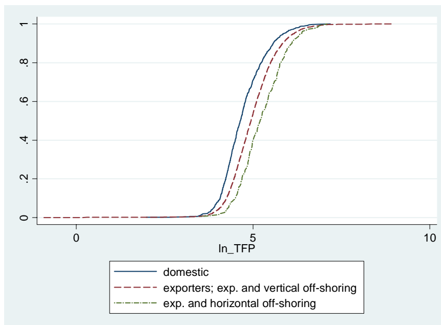
Figure 2: Plot of the cumulative distribution function of TFP: purely domestic, exporters, horizontal off-shorers (Levinsohn-Petrin method; BR classification)
