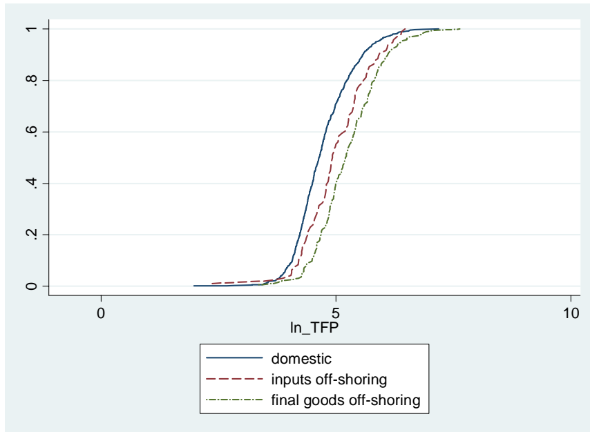
Figure 5: Plot of the cumulative distribution function of TFP: purely domestic, inputs off-shoring, final goods off-shoring (Levinsohn-Petrin method; classification based on Question D3.2.1)
