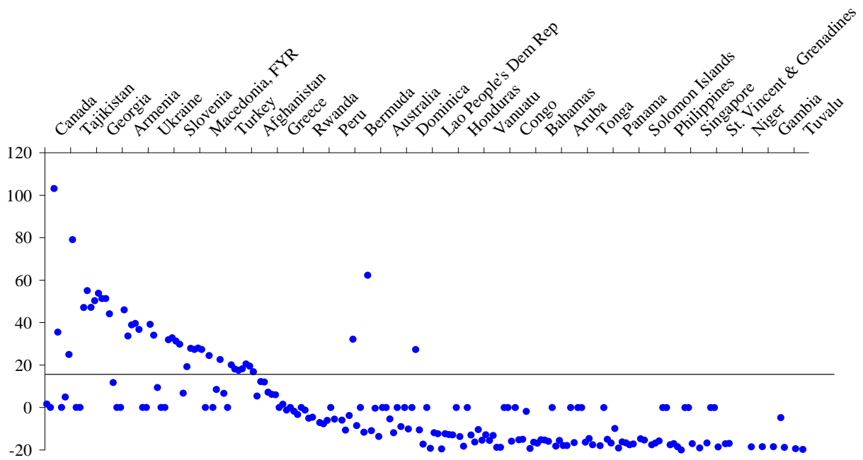
Figure 3. The effect of climate change on domestic tourist numbers, as a percentage of the numbers without climate change; top panel: world average, maximum increase (positive), and maximum decrease (negative); bottom panel: impact in 2100, countries ranked to their annual average temperature in 1961-1990.
