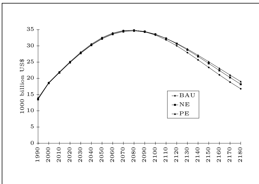
figure : Discounted consumption flows
