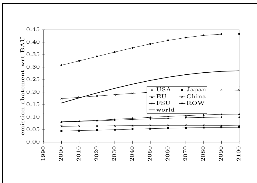
Figure 4: Nash equilibrium emission control rates
